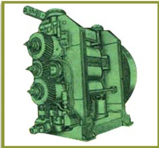
Three Roll 'I' Type Bull Gear Drive With Friction Gears
